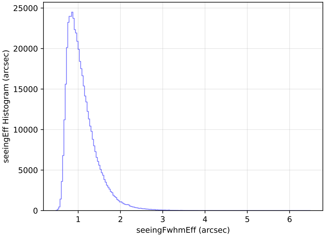
too_elab_r16_d3_gz_v3.4_10yrs All sky i band: seeingEff Histogram
