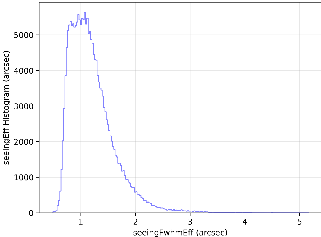
too_elab_r16_d3_gz_v3.4_10yrs All sky g band: seeingEff Histogram
