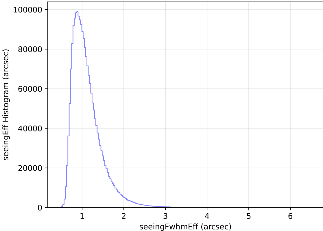
too_elab_r16_d3_gz_v3.4_10yrs All sky all bands: seeingEff Histogram
