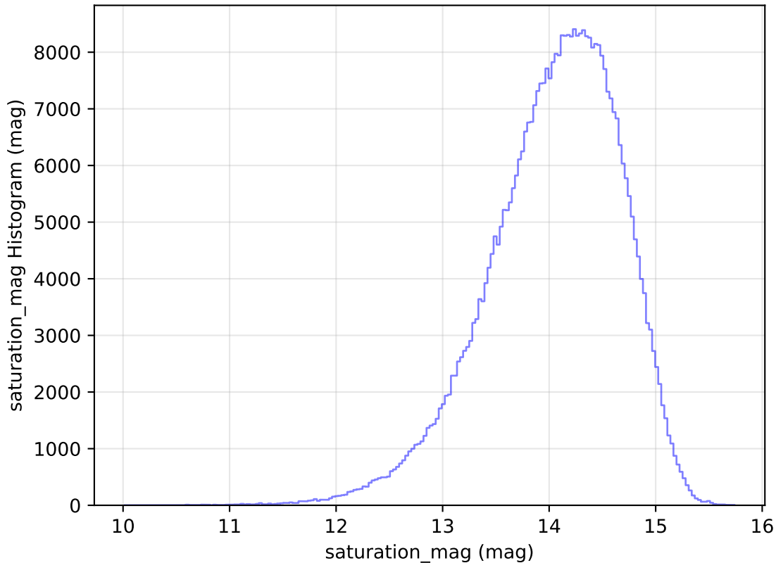
too_elab_r16_d3_gz_v3.4_10yrs WFD z band: saturation_mag Histogram
