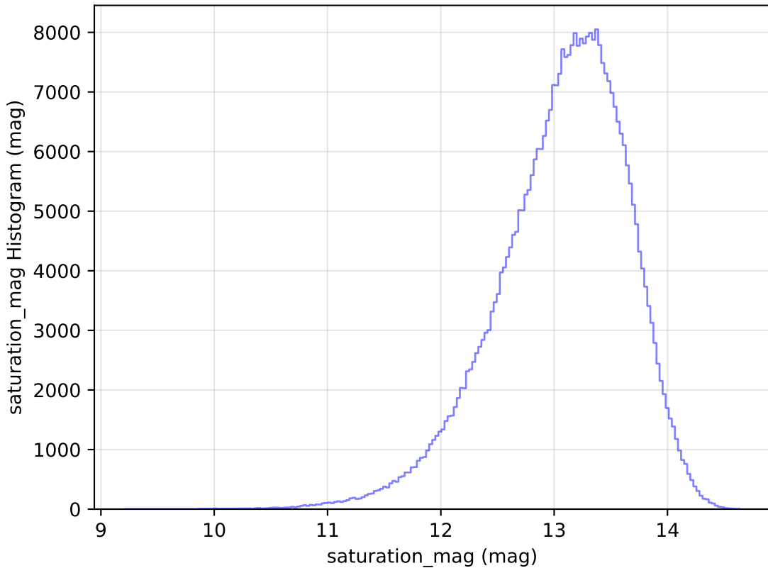
too_elab_r16_d3_gz_v3.4_10yrs WFD y band: saturation_mag Histogram
