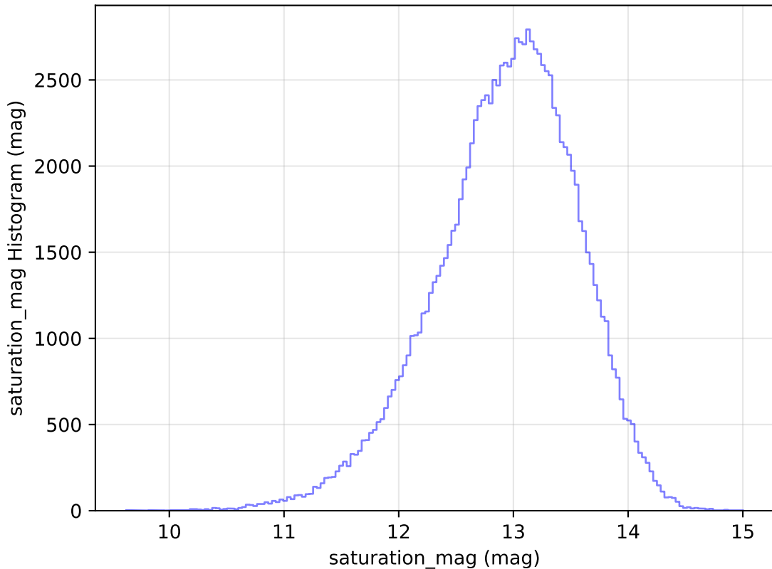
too_elab_r16_d3_gz_v3.4_10yrs WFD u band: saturation_mag Histogram
