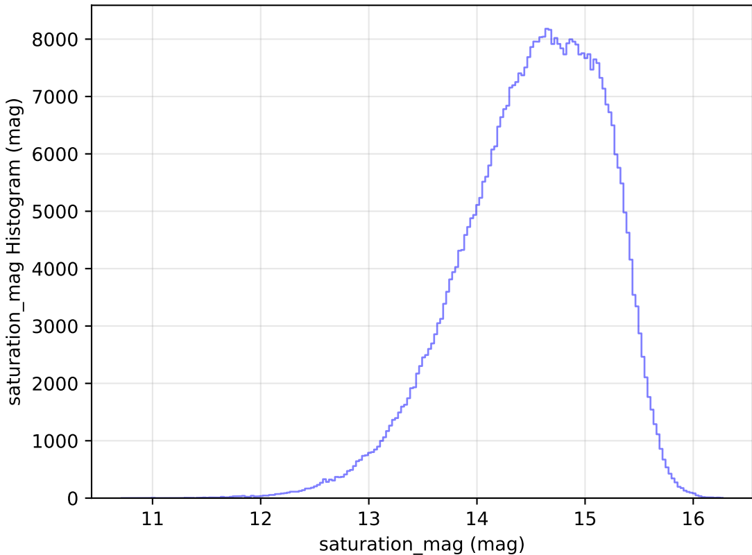
too_elab_r16_d3_gz_v3.4_10yrs WFD r band: saturation_mag Histogram
