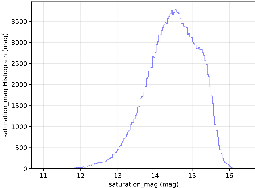
too_elab_r16_d3_gz_v3.4_10yrs WFD g band: saturation_mag Histogram
