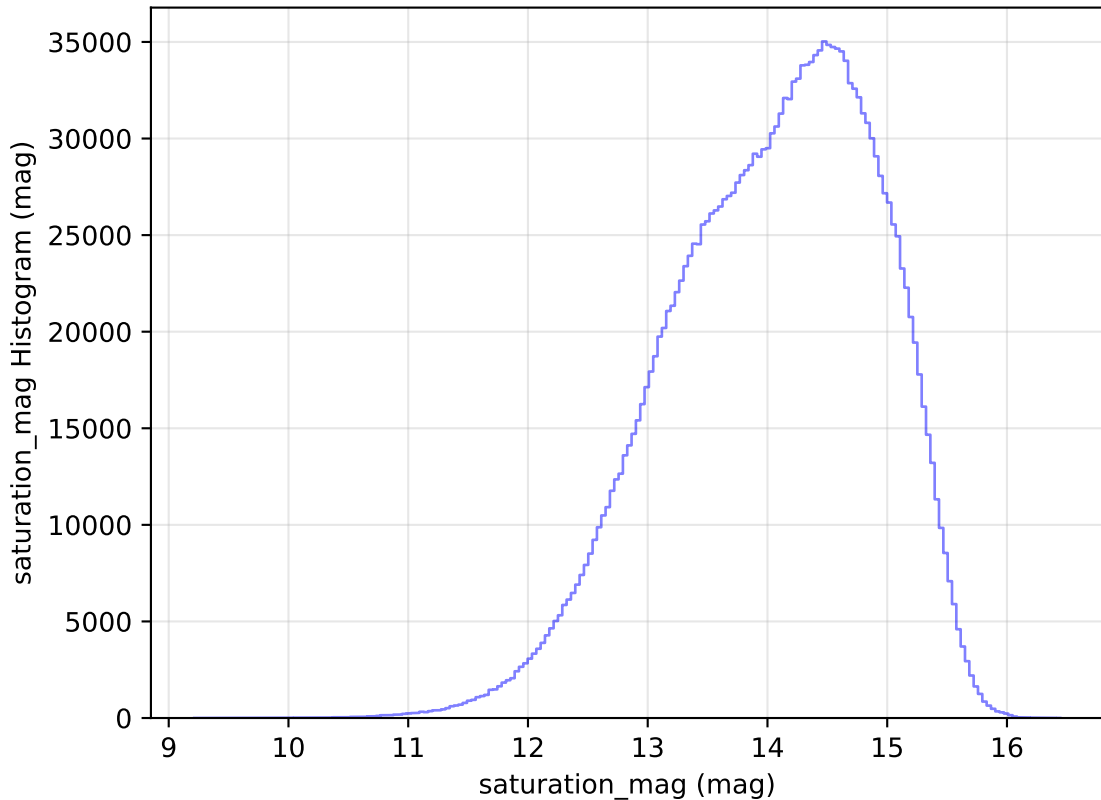
too_elab_r16_d3_gz_v3.4_10yrs WFD all bands: saturation_mag Histogram
