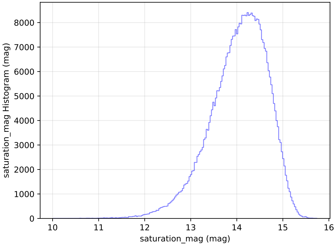
too_elab_r16_d3_gz_v3.4_10yrs All sky z band: saturation_mag Histogram
