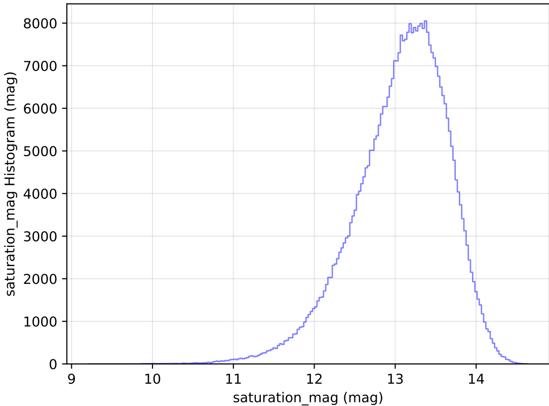
too_elab_r16_d3_gz_v3.4_10yrs All sky y band: saturation_mag Histogram
