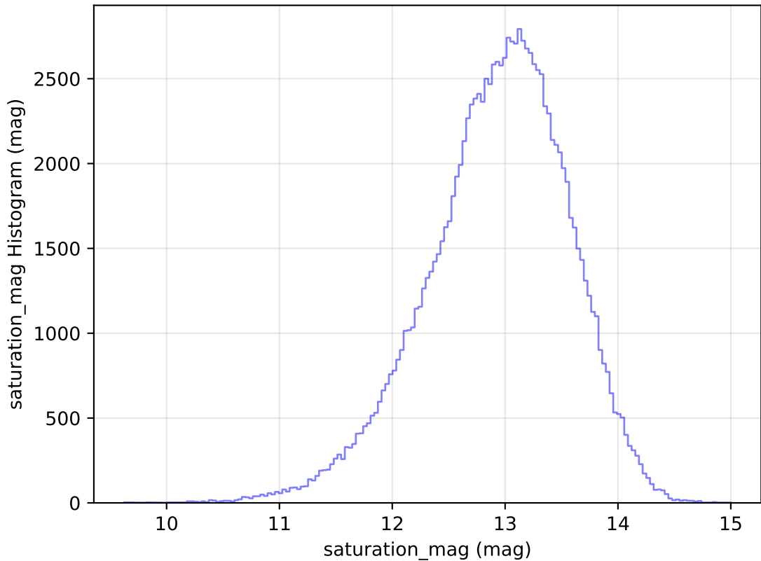
too_elab_r16_d3_gz_v3.4_10yrs All sky u band: saturation_mag Histogram
