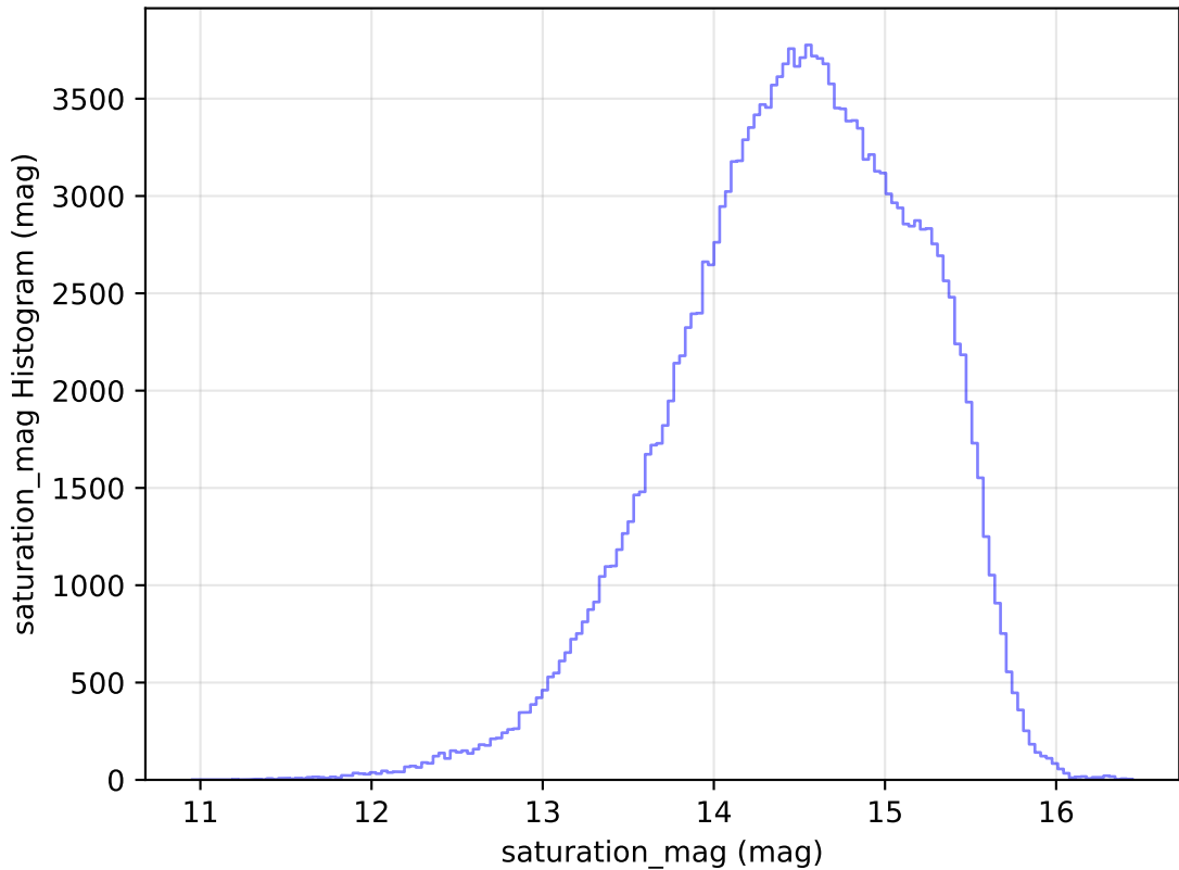
too_elab_r16_d3_gz_v3.4_10yrs All sky g band: saturation_mag Histogram
