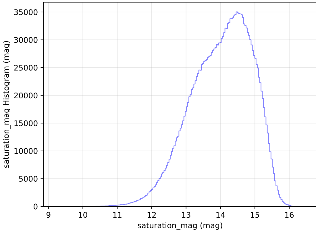
too_elab_r16_d3_gz_v3.4_10yrs All sky all bands: saturation_mag Histogram
