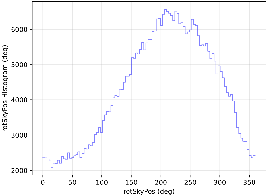
too_elab_r16_d3_gz_v3.4_10yrs WFD z band: rotSkyPos Histogram
