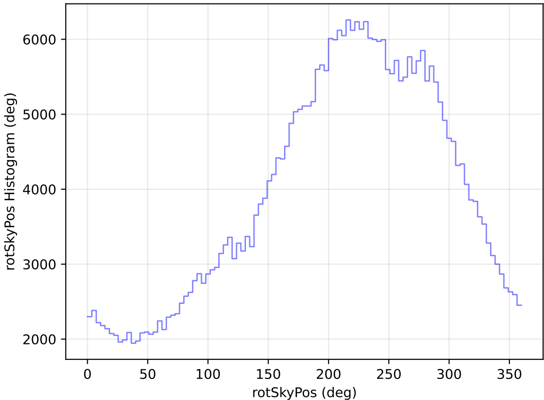
too_elab_r16_d3_gz_v3.4_10yrs WFD y band: rotSkyPos Histogram
