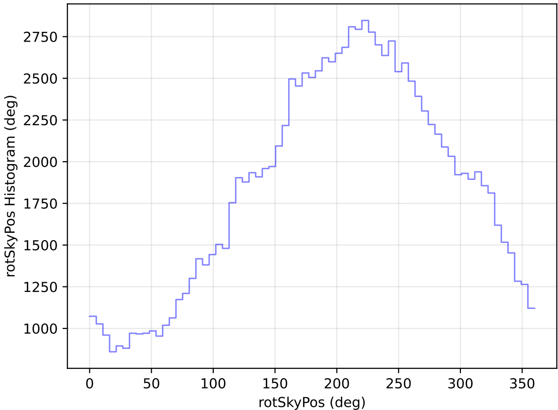
too_elab_r16_d3_gz_v3.4_10yrs WFD u band: rotSkyPos Histogram
