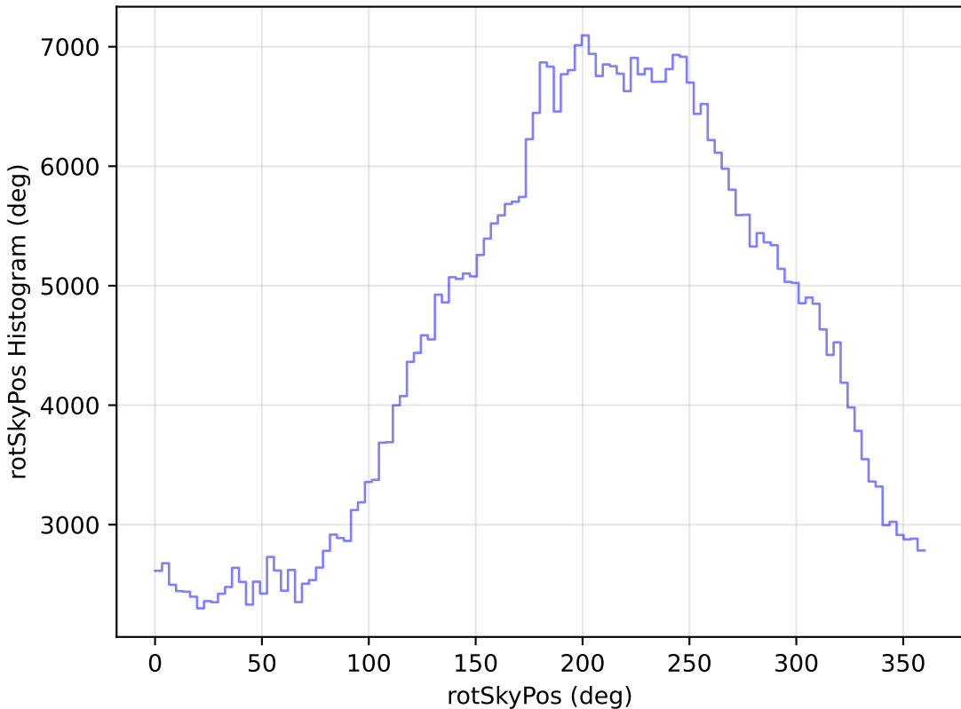
too_elab_r16_d3_gz_v3.4_10yrs WFD i band: rotSkyPos Histogram
