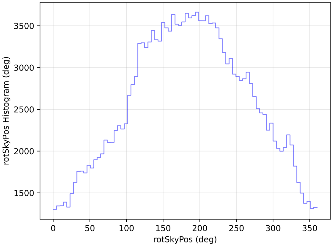
too_elab_r16_d3_gz_v3.4_10yrs WFD g band: rotSkyPos Histogram
