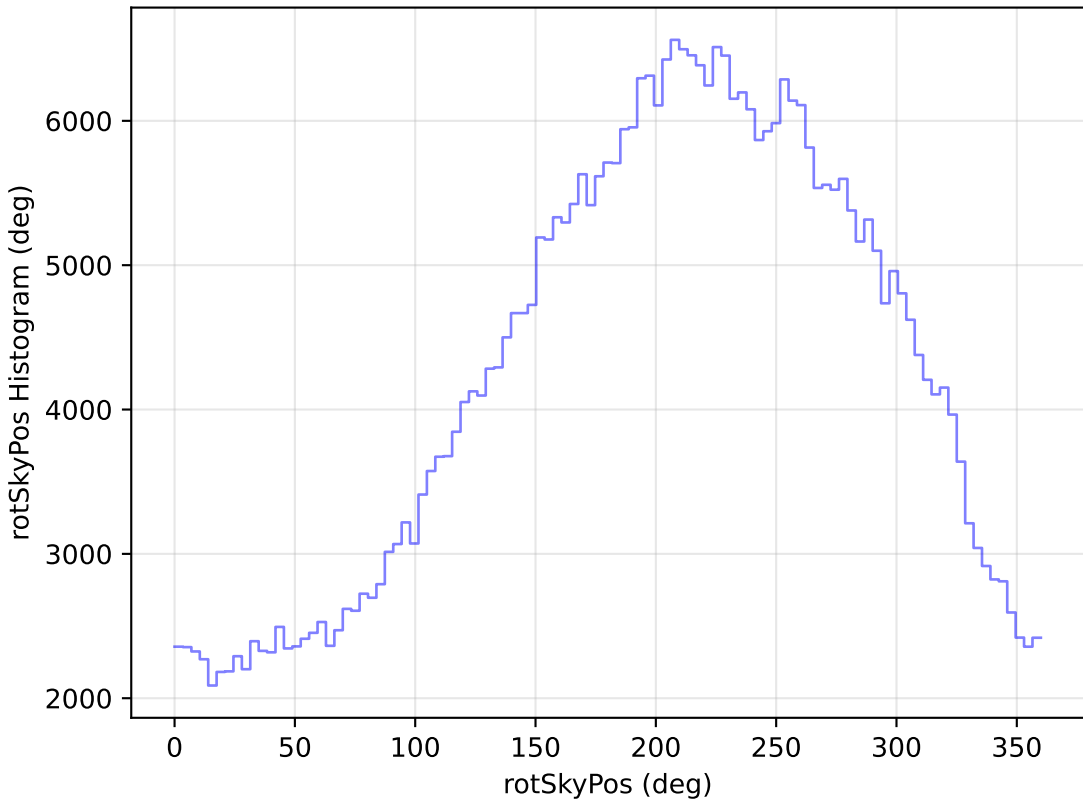
too_elab_r16_d3_gz_v3.4_10yrs All sky z band: rotSkyPos Histogram
