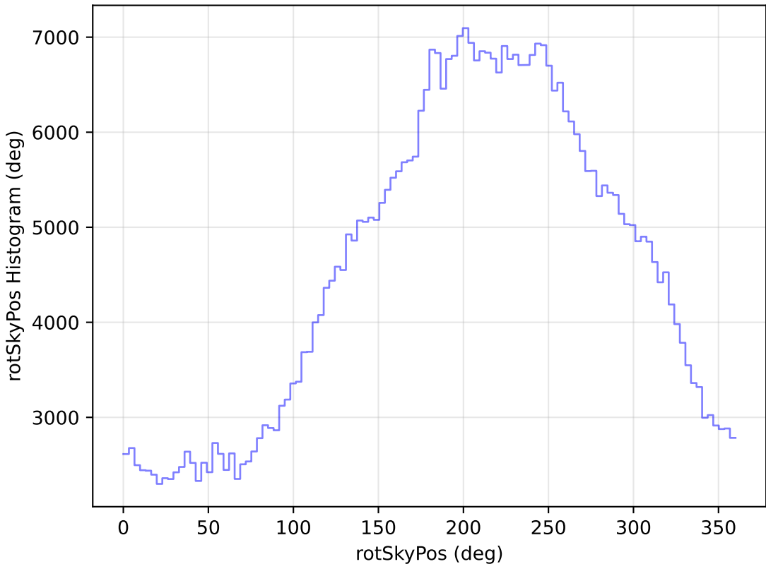
too_elab_r16_d3_gz_v3.4_10yrs All sky i band: rotSkyPos Histogram
