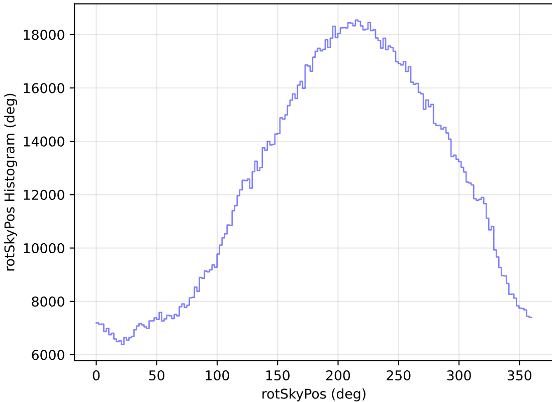
too_elab_r16_d3_gz_v3.4_10yrs All sky all bands: rotSkyPos Histogram
