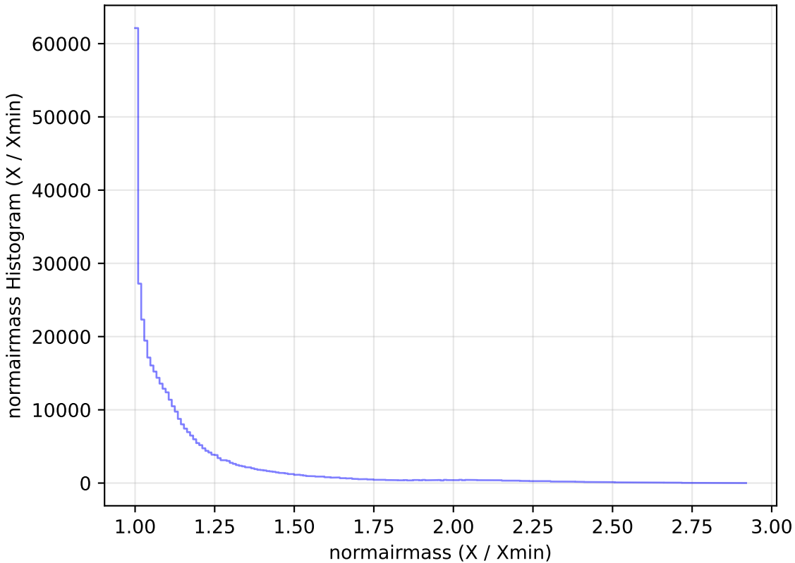
too_elab_r16_d3_gz_v3.4_10yrs WFD z band: normairmass Histogram
