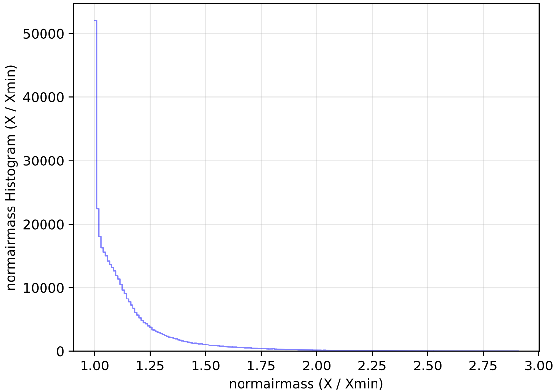
too_elab_r16_d3_gz_v3.4_10yrs WFD y band: normairmass Histogram
