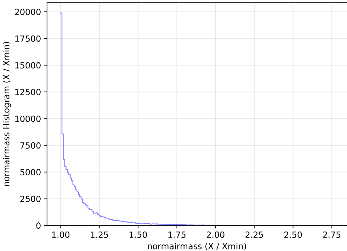
too_elab_r16_d3_gz_v3.4_10yrs WFD u band: normairmass Histogram
