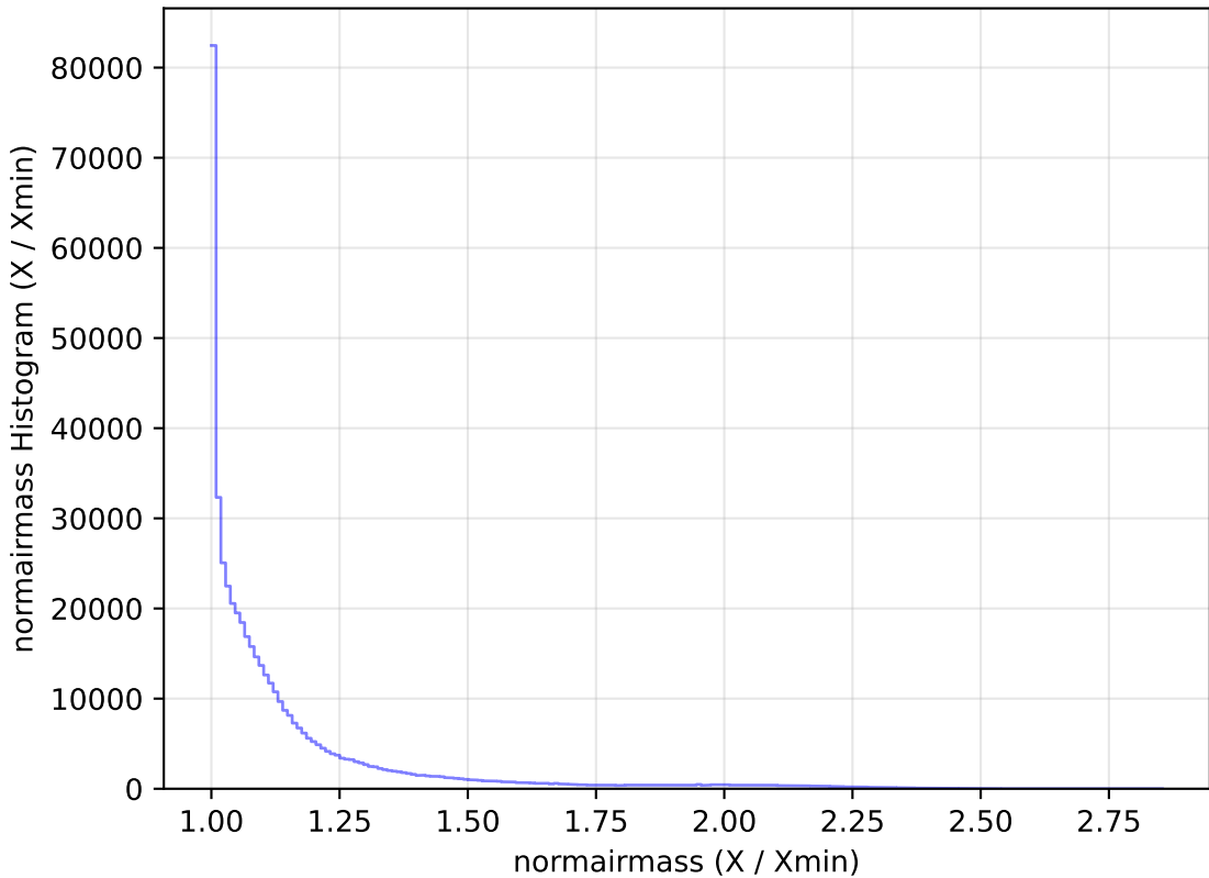
too_elab_r16_d3_gz_v3.4_10yrs WFD r band: normairmass Histogram
