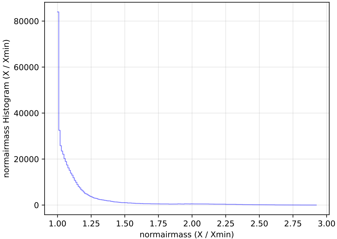
too_elab_r16_d3_gz_v3.4_10yrs WFD i band: normairmass Histogram
