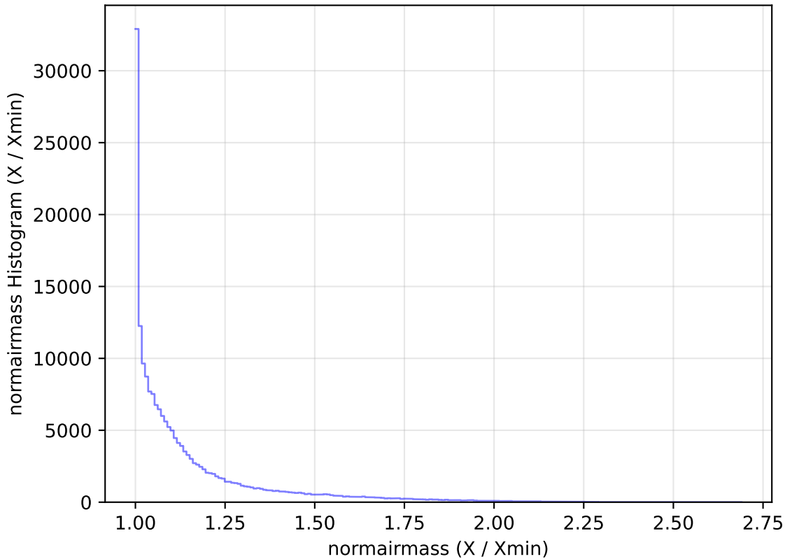
too_elab_r16_d3_gz_v3.4_10yrs WFD g band: normairmass Histogram
