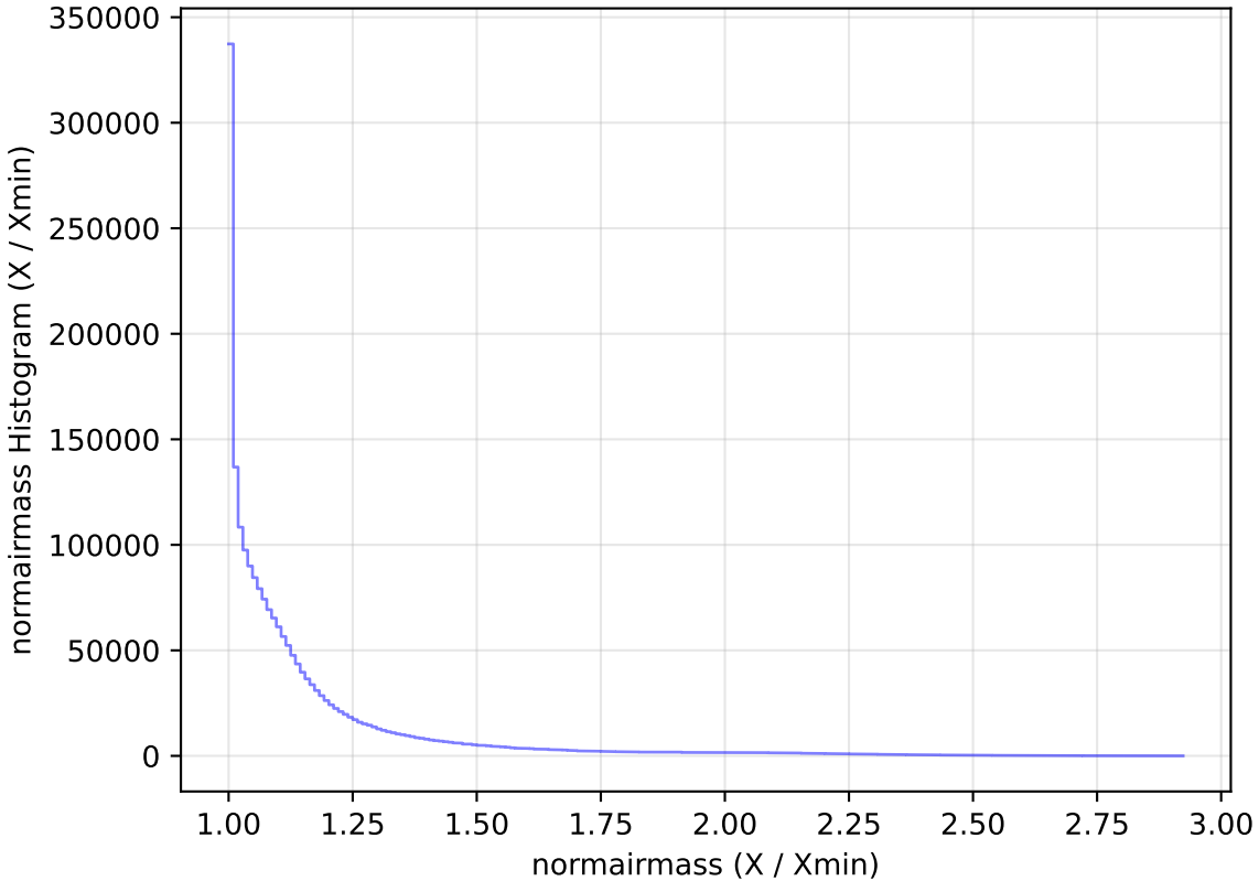
too_elab_r16_d3_gz_v3.4_10yrs WFD all bands: normairmass Histogram
