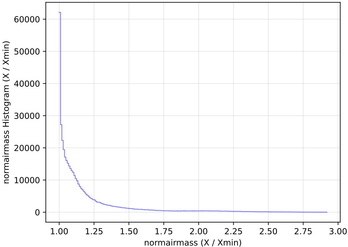
too_elab_r16_d3_gz_v3.4_10yrs All sky z band: normairmass Histogram
