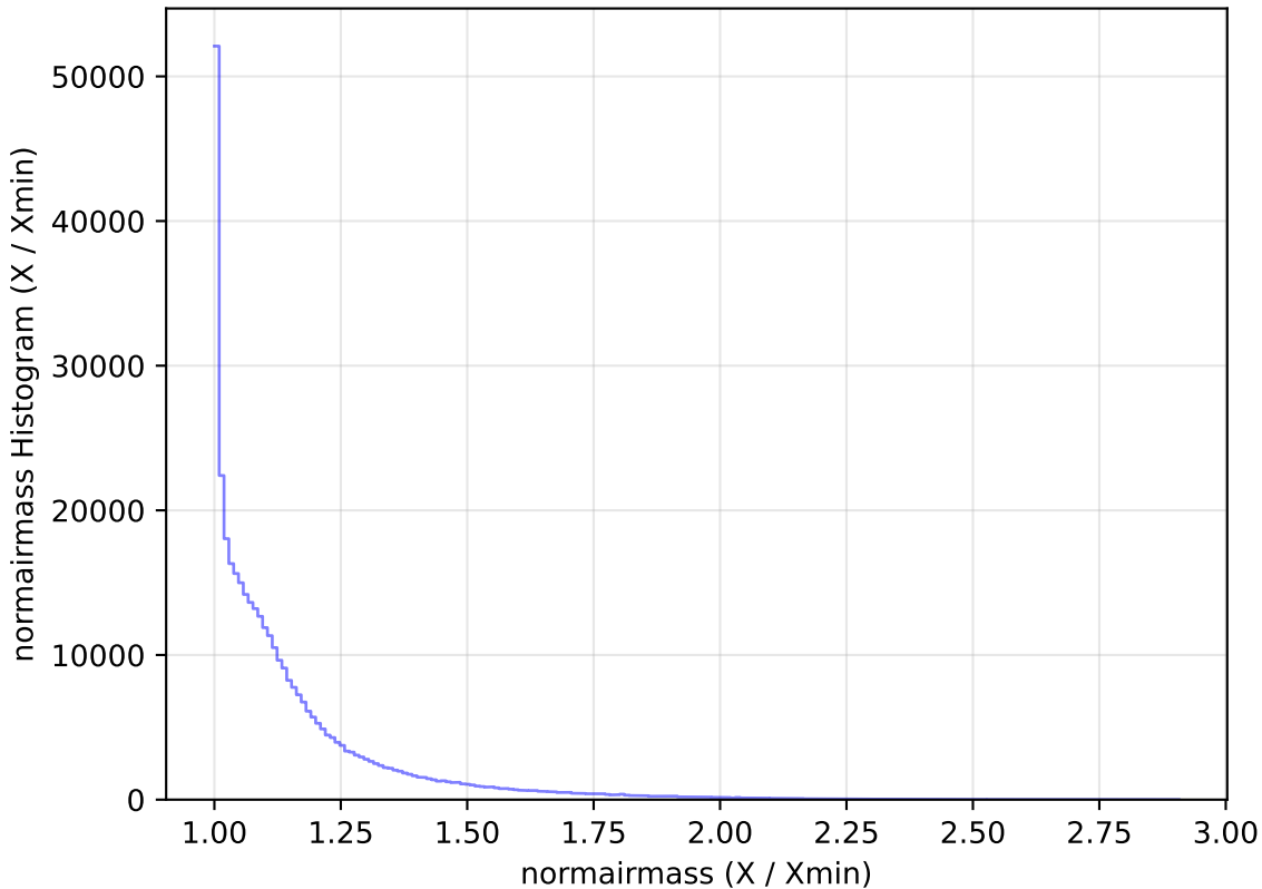
too_elab_r16_d3_gz_v3.4_10yrs All sky y band: normairmass Histogram
