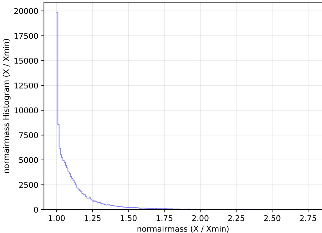
too_elab_r16_d3_gz_v3.4_10yrs All sky u band: normairmass Histogram
