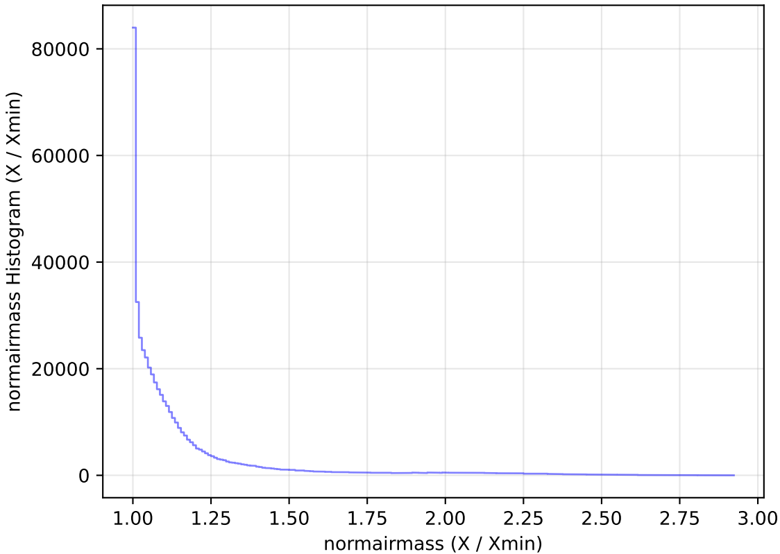
too_elab_r16_d3_gz_v3.4_10yrs All sky i band: normairmass Histogram
