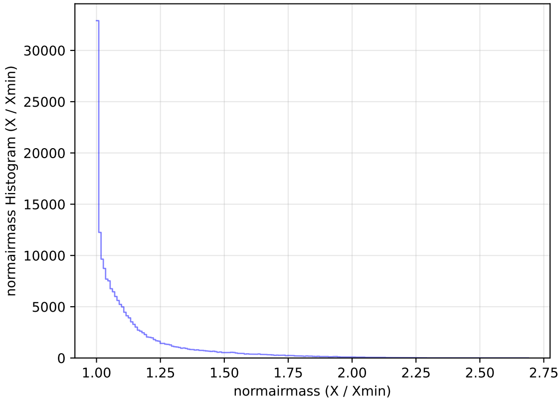
too_elab_r16_d3_gz_v3.4_10yrs All sky g band: normairmass Histogram
