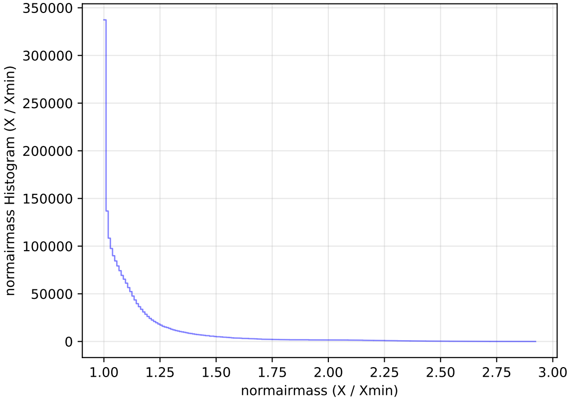
too_elab_r16_d3_gz_v3.4_10yrs All sky all bands: normairmass Histogram
