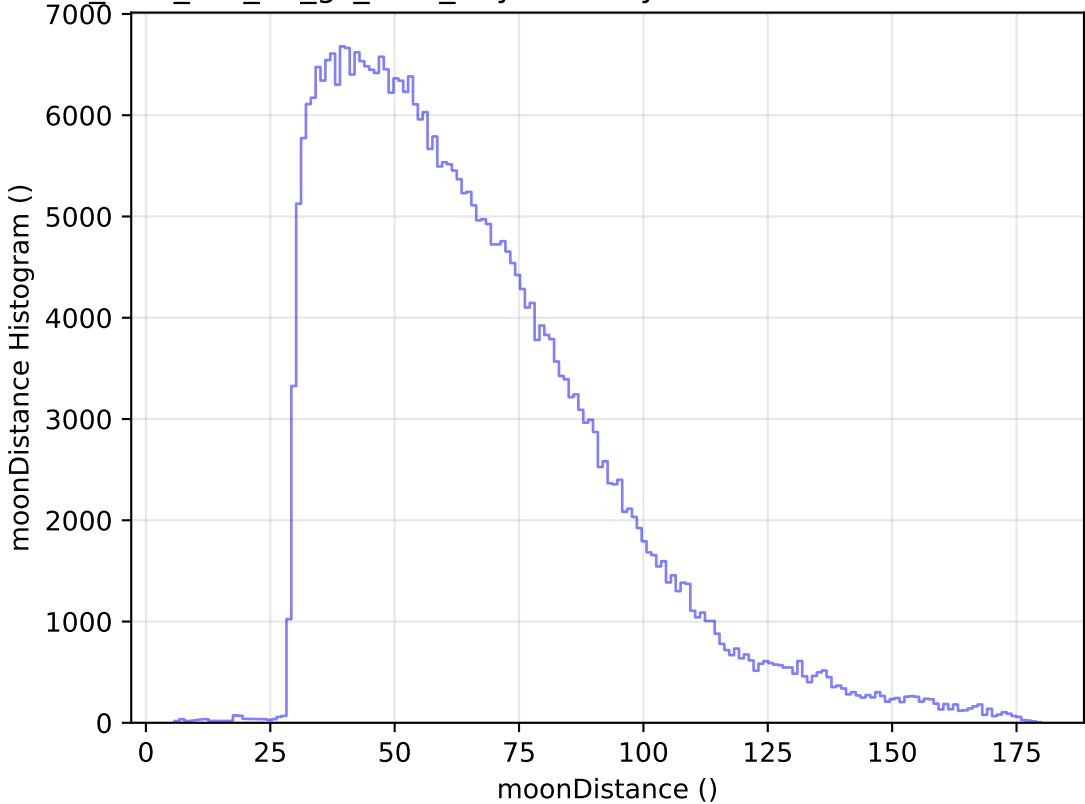
too_elab_r16_d3_gz_v3.4_10yrs WFD y band: moonDistance Histogram
