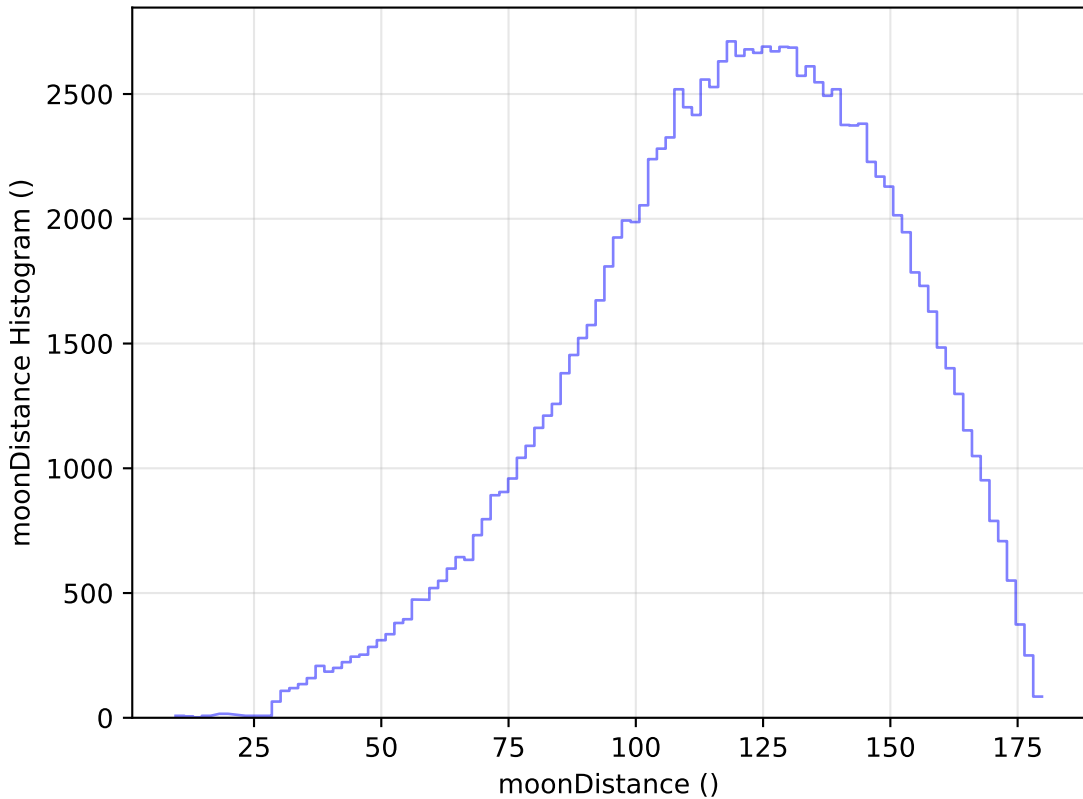
too_elab_r16_d3_gz_v3.4_10yrs WFD u band: moonDistance Histogram
