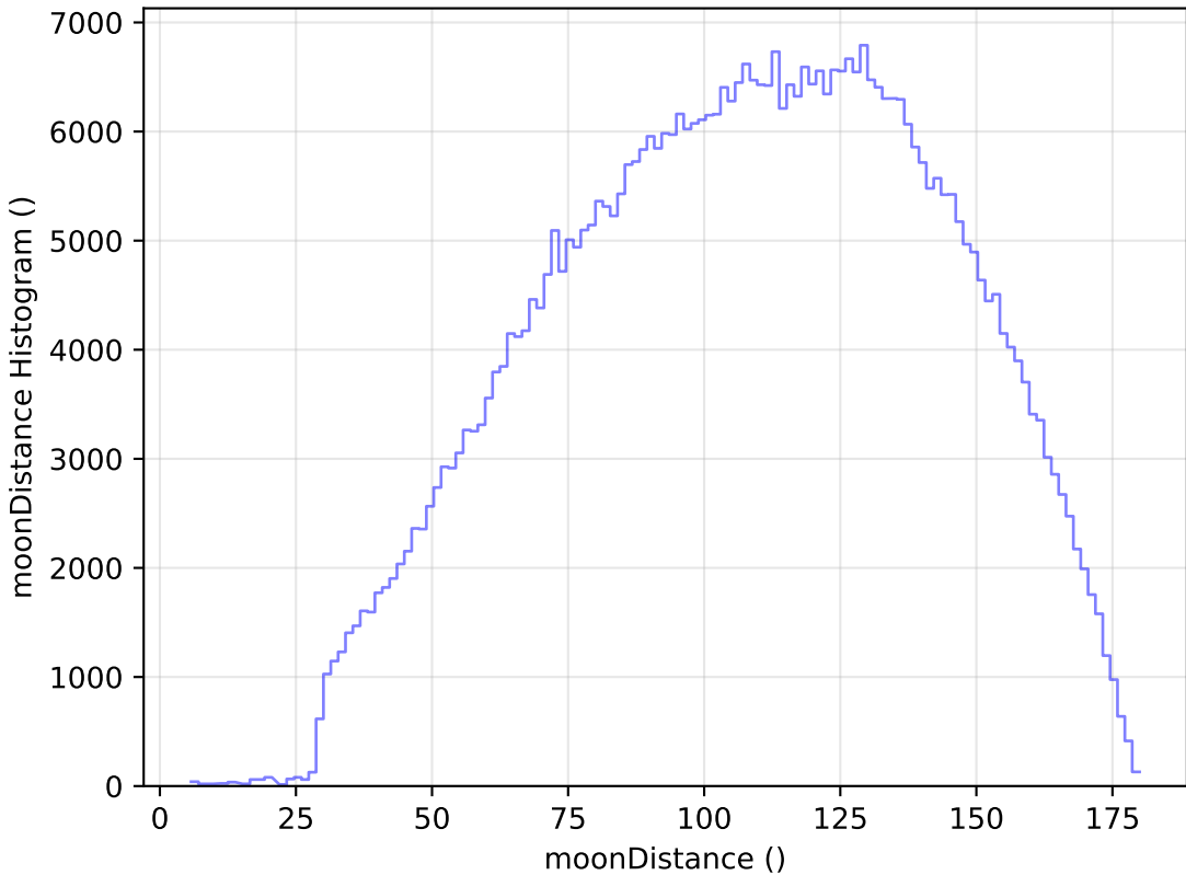
too_elab_r16_d3_gz_v3.4_10yrs WFD r band: moonDistance Histogram
