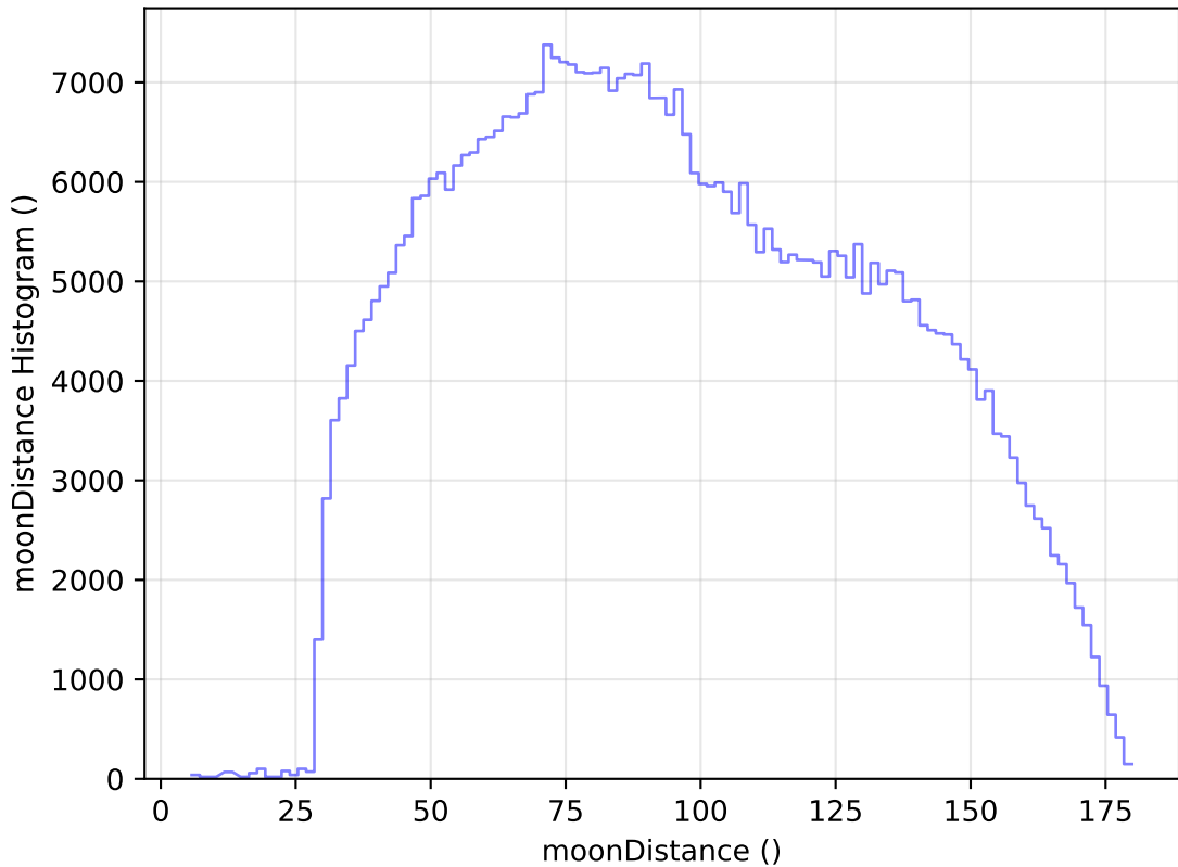
too_elab_r16_d3_gz_v3.4_10yrs WFD i band: moonDistance Histogram
