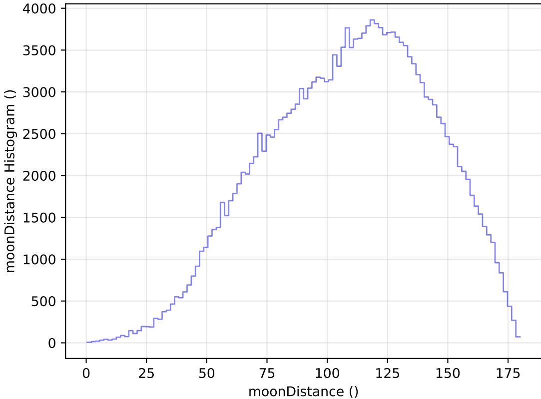
too_elab_r16_d3_gz_v3.4_10yrs WFD g band: moonDistance Histogram
