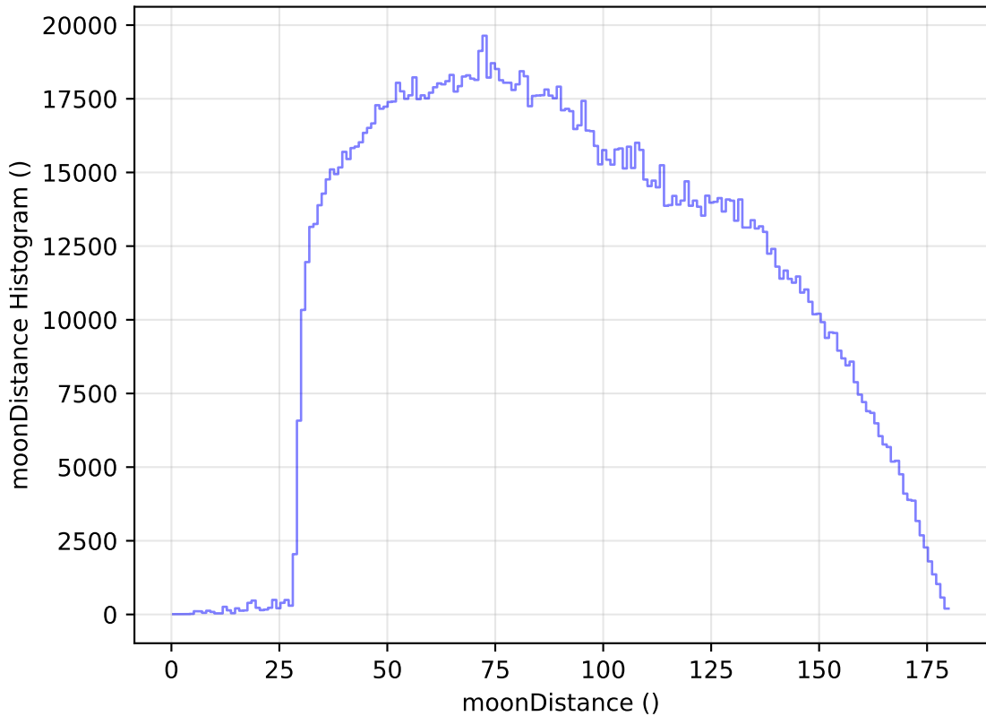
too_elab_r16_d3_gz_v3.4_10yrs WFD all bands: moonDistance Histogram
