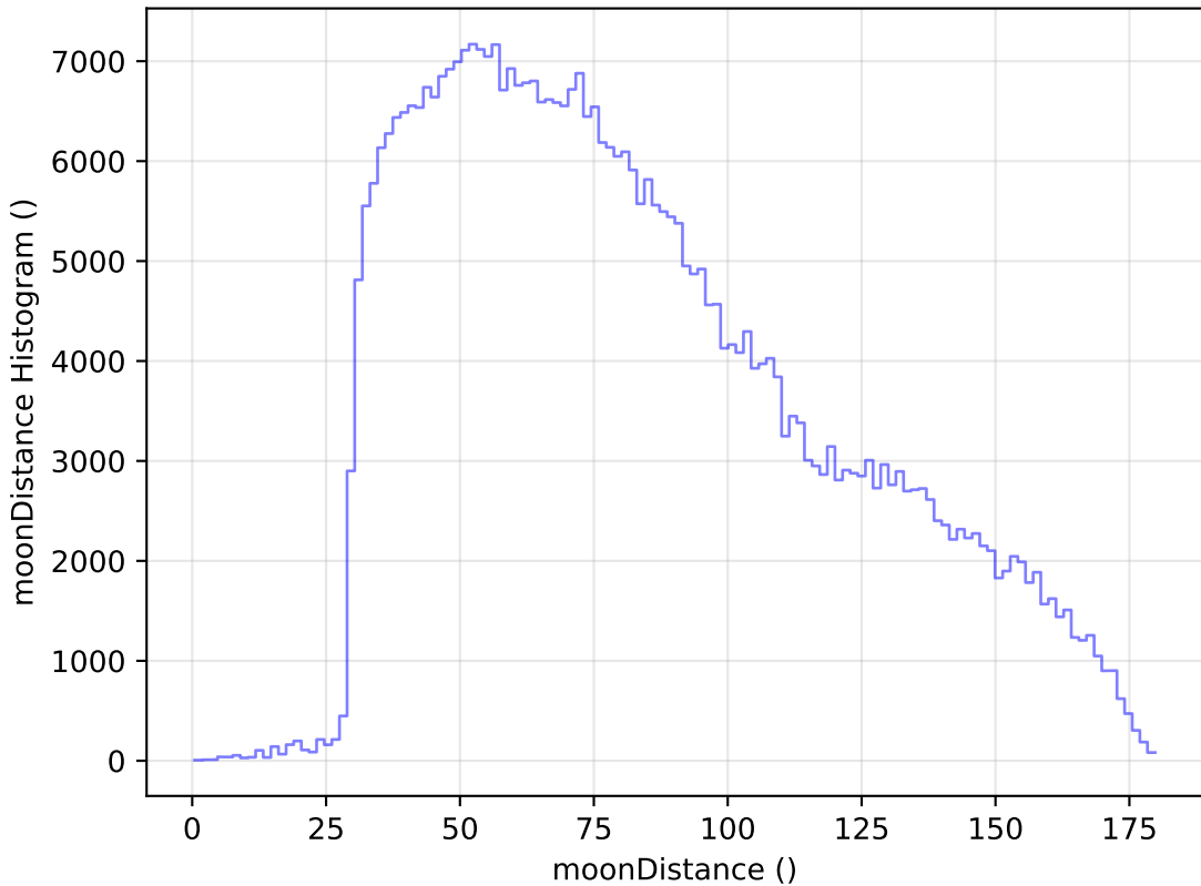
too_elab_r16_d3_gz_v3.4_10yrs All sky z band: moonDistance Histogram
