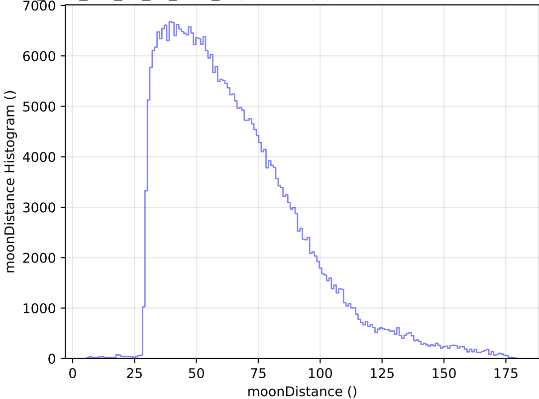
too_elab_r16_d3_gz_v3.4_10yrs All sky y band: moonDistance Histogram
