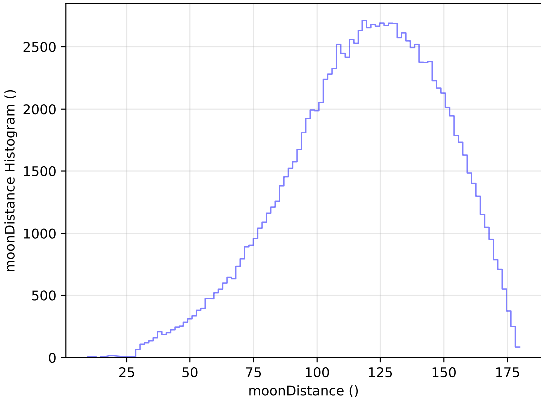
too_elab_r16_d3_gz_v3.4_10yrs All sky u band: moonDistance Histogram
