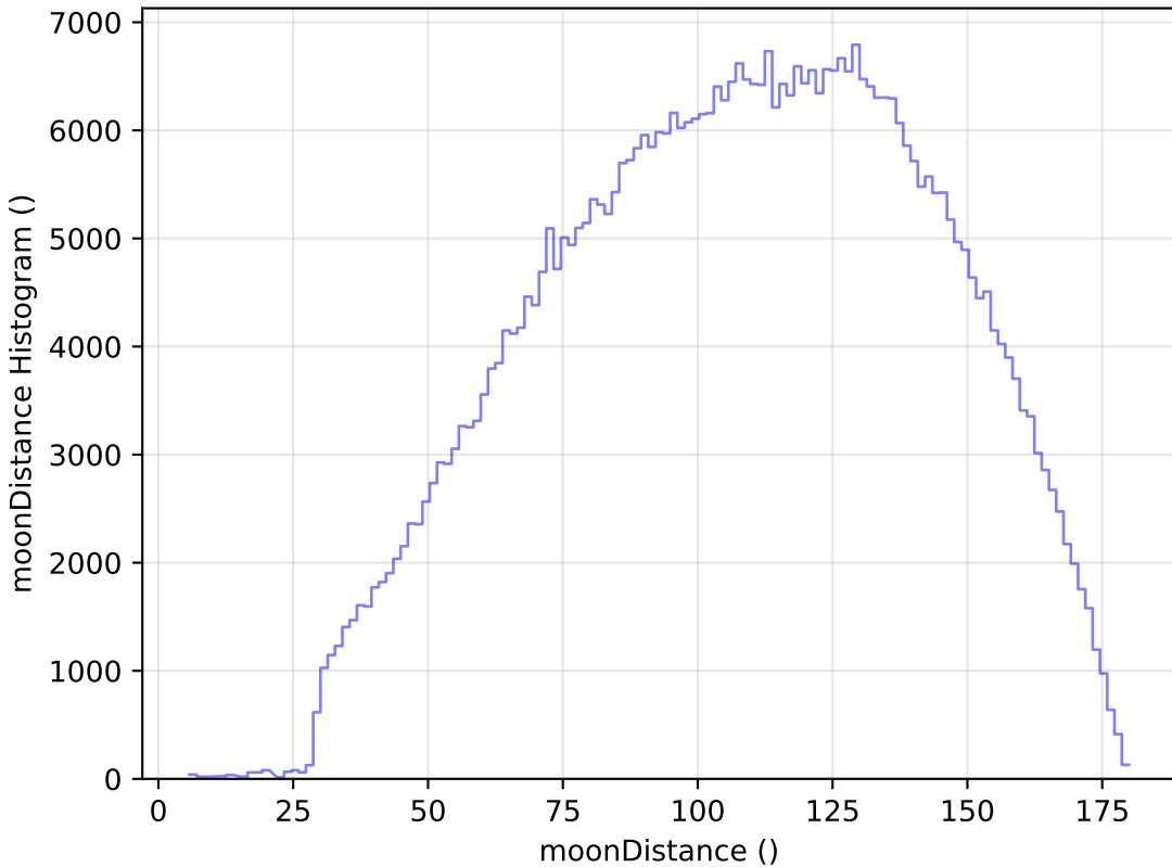
too_elab_r16_d3_gz_v3.4_10yrs All sky r band: moonDistance Histogram
