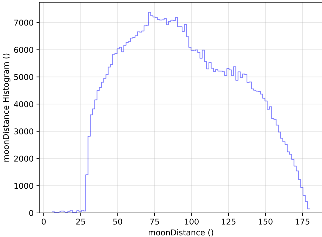
too_elab_r16_d3_gz_v3.4_10yrs All sky i band: moonDistance Histogram
