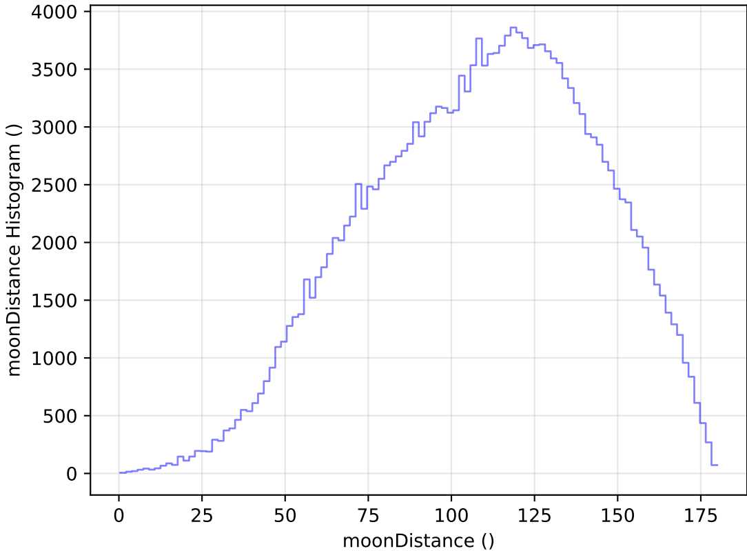
too_elab_r16_d3_gz_v3.4_10yrs All sky g band: moonDistance Histogram
