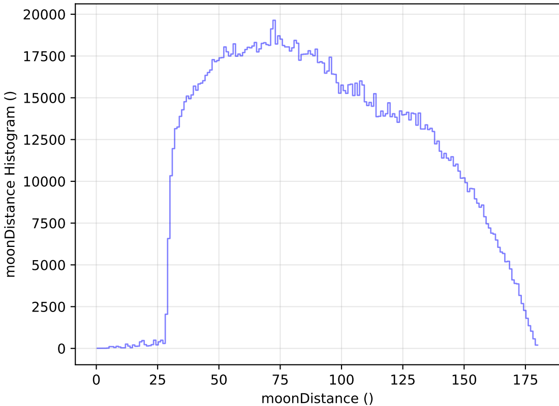
too_elab_r16_d3_gz_v3.4_10yrs All sky all bands: moonDistance Histogram
