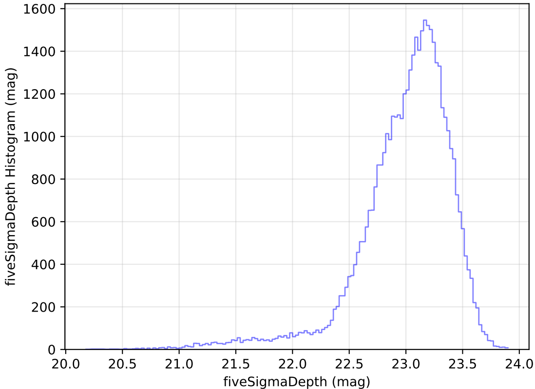
too_elab_r16_d3_gz_v3.4_10yrs Yr 1 z band: fiveSigmaDepth Histogram
