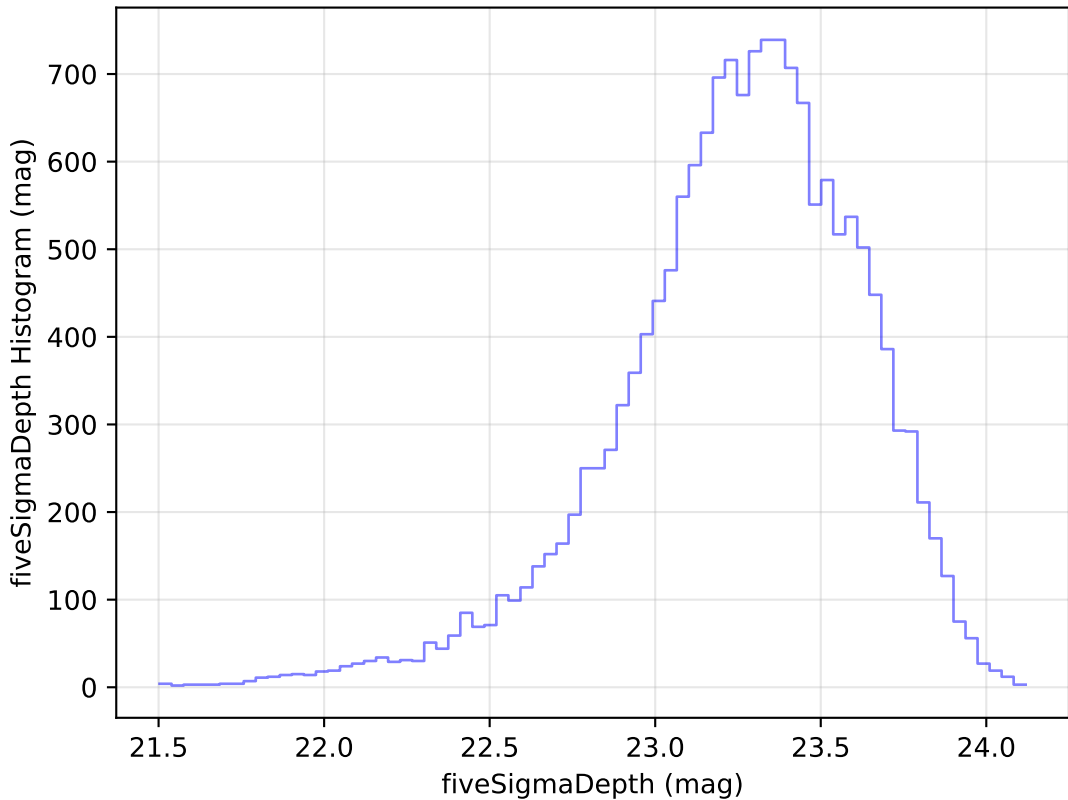
too_elab_r16_d3_gz_v3.4_10yrs Yr 1 u band: fiveSigmaDepth Histogram
